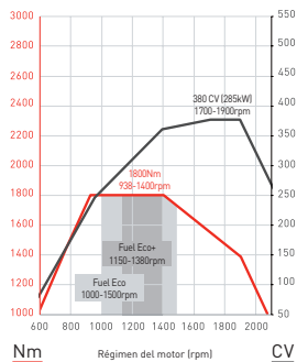
DE11 - 380 CV
