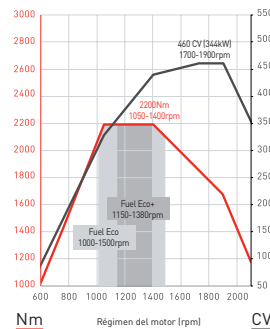
DE11 - 460 CV
