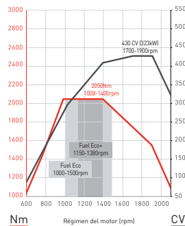
DE11 - 430 CV
